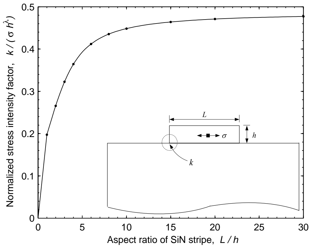
FIG. 2. The normalized stress intensity factor, k/(\sigma h^\lambda) , calculated using a finite element method, is shown as a function of the aspect ratio, L/h , of the nitride stripe.
